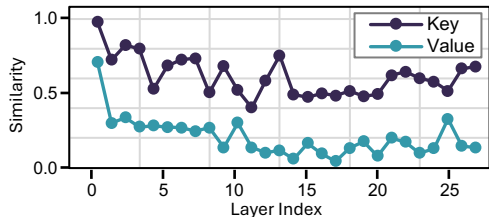
(b) Static Patch Similarity Comparison
