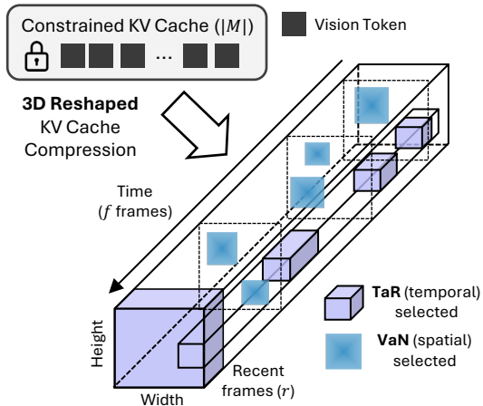
(a) Temporal-axis Redundancy Reduction (TaR)
