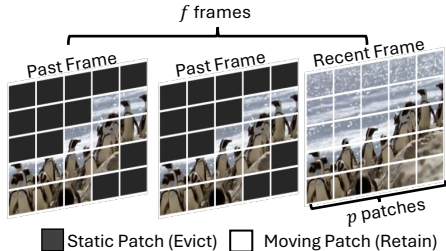
(a) Temporal-axis Redundancy Reduction (TaR)
